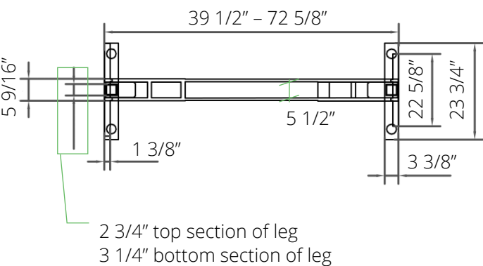
T33M Height adjustable base dimensions
