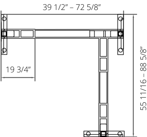
T33M Height adjustable base dimensions
